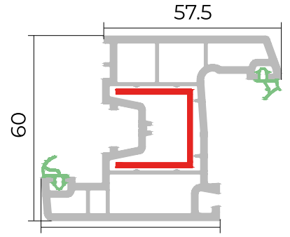
Qanad profili Sash profile
