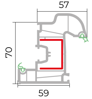
Dekorativ qanad profili Decorative sash profile
