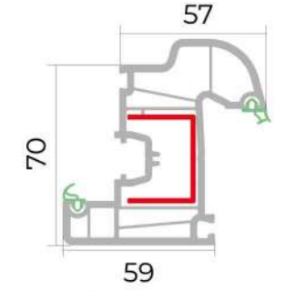
Dekorativ qanad profili Decorative sash profile
