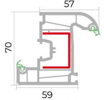
Qanad profili Sash profile
